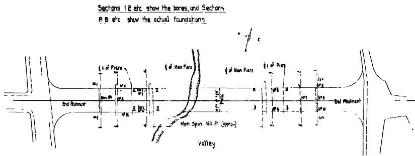
Fig. 15.—Site Plan of Bridge showing Position of Bores.
